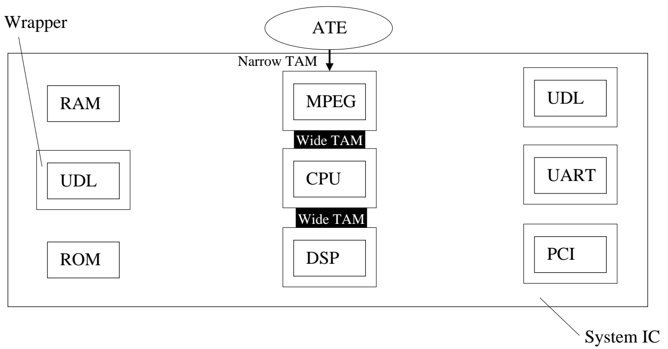
Figure 1. Test architecture of MILET.
